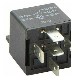
Standard Relay SPDT (Single Pole Double Throw)
